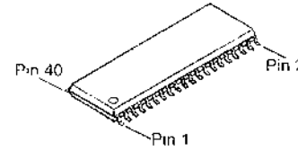
M5M82C55AFP (Q5023, 50228, 5029, 5030)
