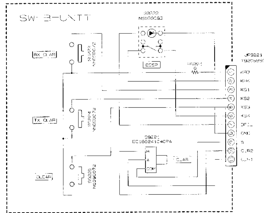
SW-B Unit Circuit Diagram
