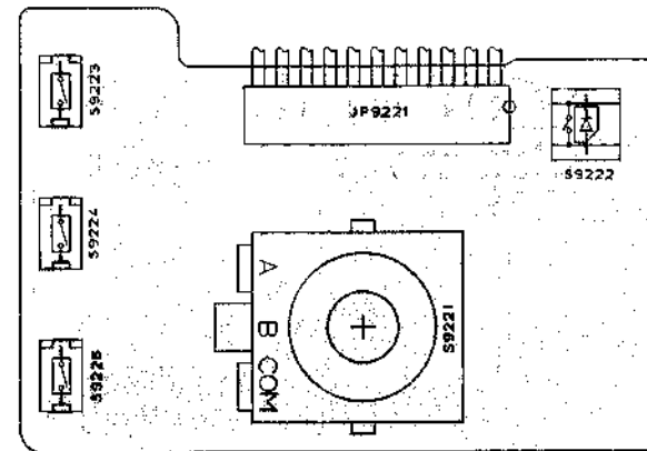
SW-B Unit Parts Layout
