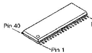
M5M82C55AFP (Q5023, 50228, 5029, 5030)
