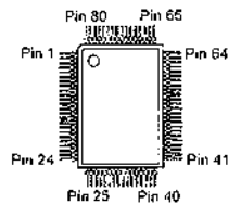
M37702E8BFP (Q5008)
